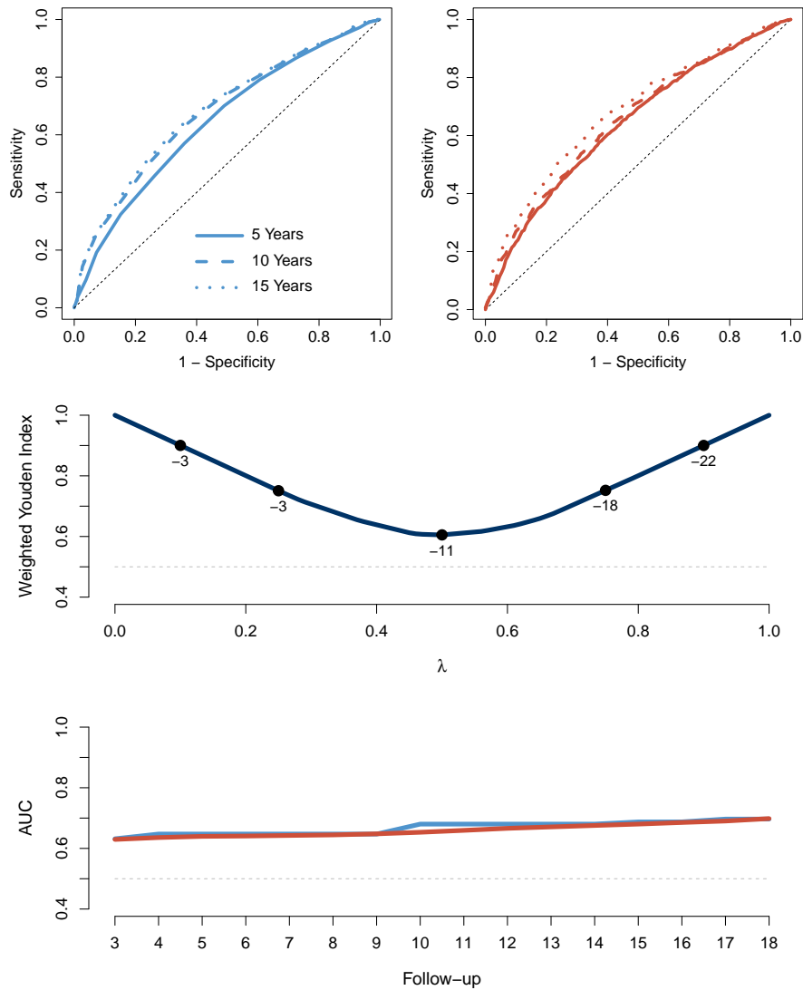
Figure 3: Top: ROC curves estimates at 5, 10 and 15 years from the sMSROC (left), and from the cenROC (right) packages. Middle: Weighted Youden Index at 5 years from the sMSROC curve estimation. Bottom: AUC evolution from 3 to 18 years for the two considered estimators.
