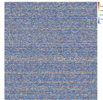
(c) Heatmap of simulated dataset. 15K entities, 100 categories. Colors according to value of abundance.
