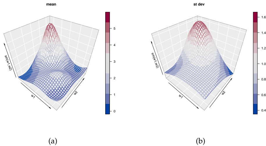
Figure 4: Bivariate simulation study results with two continuous covariates. Posterior means of the (a) mean and (b) standard deviation function.
