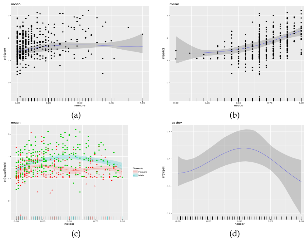
Figure 7: Results from the data analysis on the relationship between covariates gender, marital status, experience, education and tenure, and response variable logarithm of hourly wage. Posterior means and 95% credible intervals for (a) f_1(\text{ntenure}) , (b) f_2(\text{neduc}) , (c) f_3(\text{nexper}, \text{female}) , and (d) the standard deviation function \sigma_i = \sigma \exp[f_4(\text{nexper})/2] .
