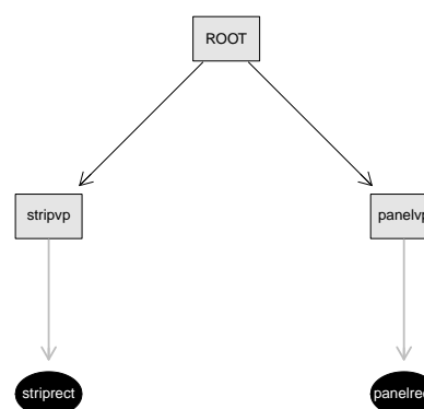
Figure 6: A node-and-edge graph of the scene from Figure 1. Both viewports are direct descendants of the ROOT viewport and one grob is drawn in each viewport.
