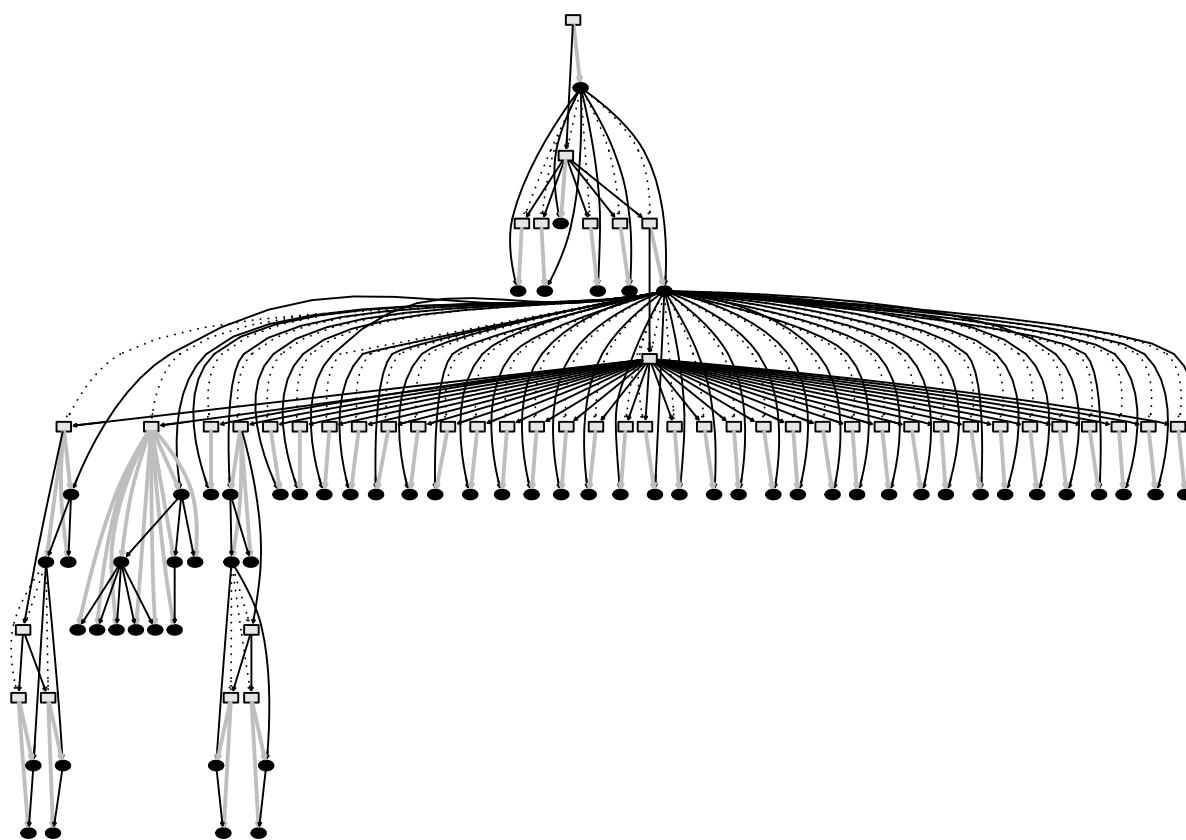
Figure 15: A node-and-edge graph of the scene from Figure 14. This scene graph was produced using ggplot2 version 0.8.9. More recent versions of ggplot2 will produce a different scene graph.
