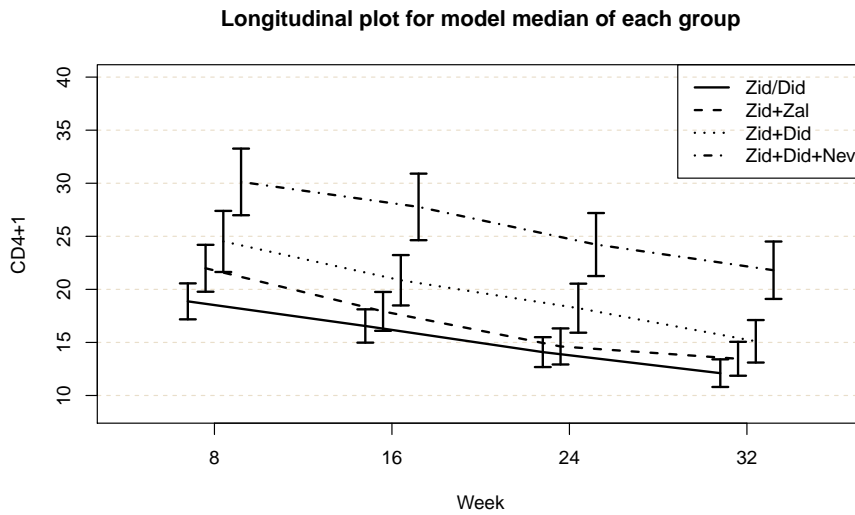
Figure 2: Longitudinal plot of model median for each group, created by applying plot function to bcmmrm object.
