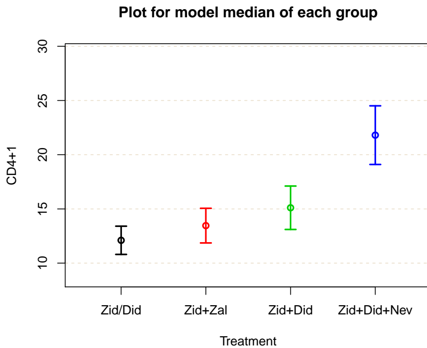
Figure 3: Plot of model median for each group at week 32, created by applying plot function to bcmmrm object with timepoint option.
